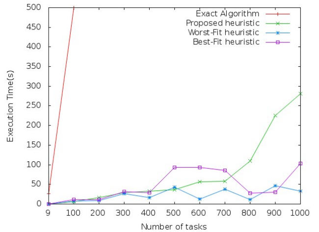
Figure 3. Execution time of the algorithms according to the number of tasks
